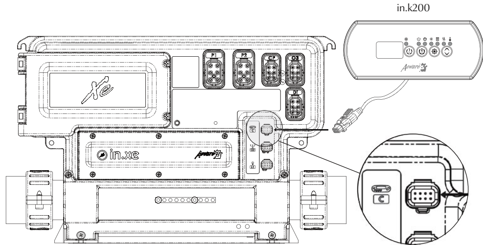
Connect the main keypad in.k200 as indicated here.
